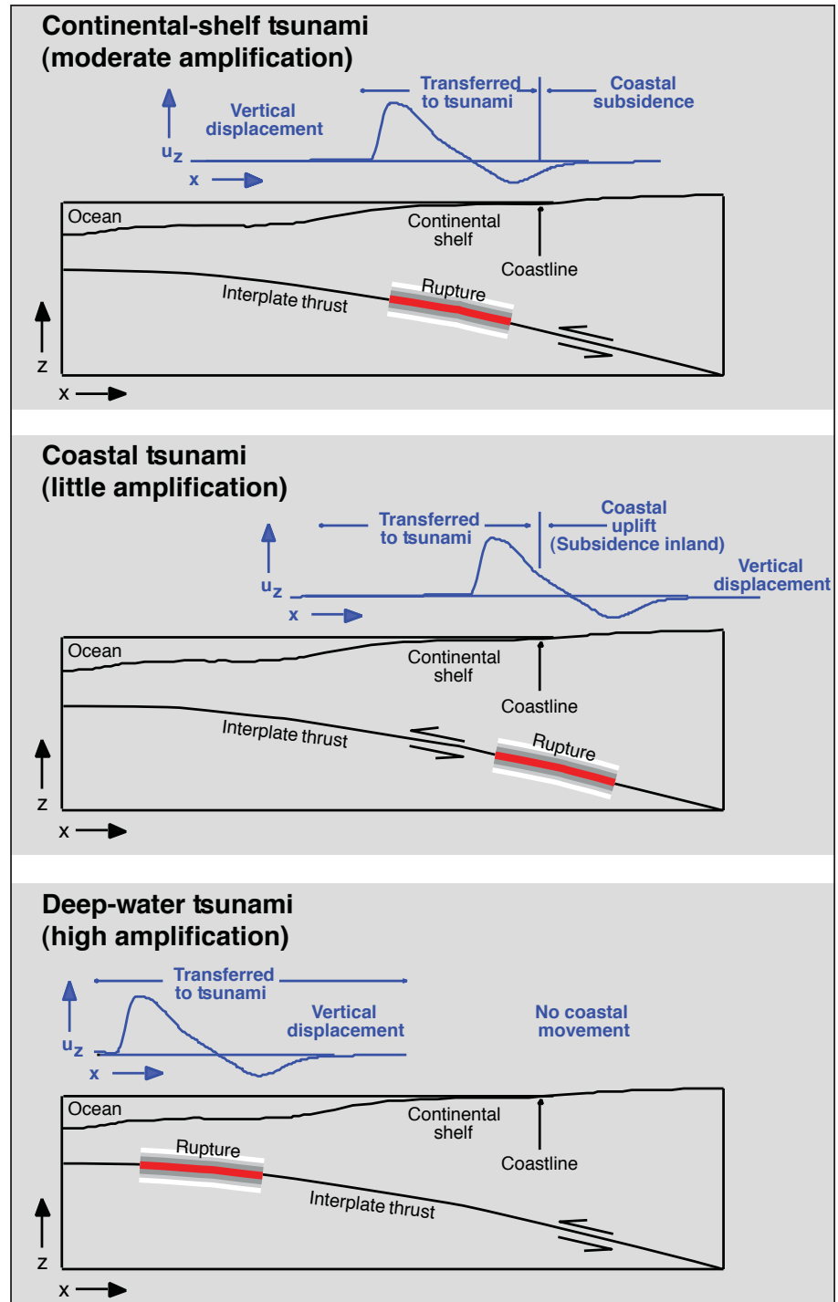
Three schematic examples showing how the location of earthquake rupture affects tsunami generation. See text (page 5) for discussion. x , horizontal distance; z , vertical distance; u_z , change in vertical distance. The oceanic trench, where the interplate thrust intersects the ocean floor, is outside the figure, to the left of each panel.
