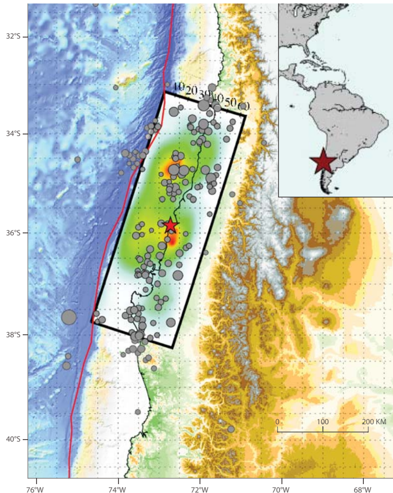
Slip pattern for the 2010 Chilean earthquake. Black rectangle encloses area on the Earth's surface directly above the section of the interplate thrust fault that ruptured during the February 27 earthquake; green shading, low to moderate slip; red shading, high slip of as much as 14 m (46 ft). Red line offshore is fault's surface trace, the line along which the fault intersects the seafloor. (The fault dips east below Chile.) Red star is the earthquake's epicenter (point on the Earth's surface directly above the earthquake's focus, or point where rupture began); gray dots are aftershock epicenters, with size proportional to magnitude. Offshore bathymetry (blue-white) and onland topography (green-tan) shown in background. Inset map shows general location of earthquake (star). Modified from Finite Fault Model from the USGS National Earthquake Information Center (NEIC): http://earthquake.usgs.gov/earthquakes/eqinthenews/2010/us2010tfan/finite_fault.php . See text (page 5) for discussion.
