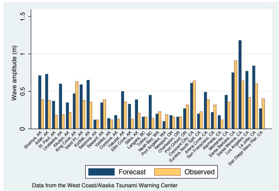
Comparison of forecasted and observed maximum Chilean 2010 tsunami amplitudes (heights above sea surface) at tide-gauge sites along the west coast of North America. Data from http://wcatwc.arh.noaa.gov/chile/chileamp.php .
